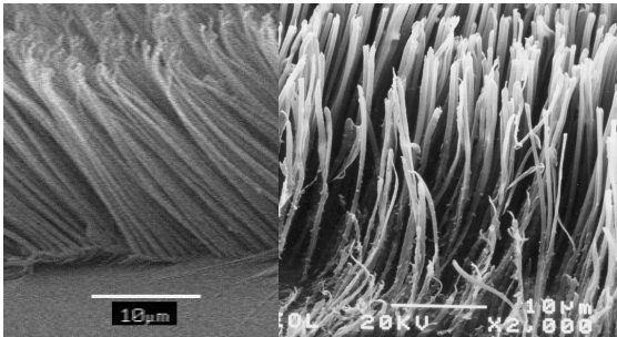
Figure 11. (left) Setae of the Anolis Equestris, length 23um, diameter 0.5um. Anoles such as this have unbranched setae with a spatula tip. (right) Polyimide fiber array synthesized using Millipore Isopore filters, length 22um, diameter 0.6um. A. Equestris image courtesy Anne Peattie.
