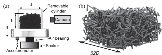
FIG. 1. Experiment and simulation of u -particle ensembles. (a) Freestanding vertical columns are formed on a vibration table and the collapse dynamics are observed under vertical vibration. (b) Computer generated ensembles of u particles.
